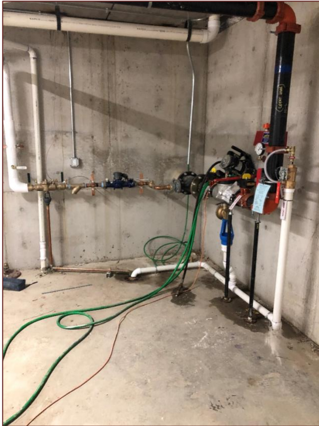
Fire suppression system.
